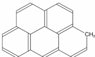
Kinolin
